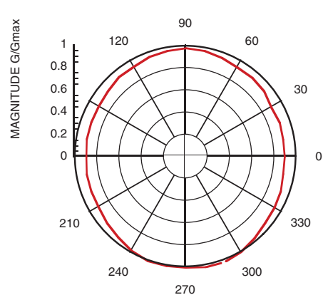
Linear Gain vs. Phase Setting
