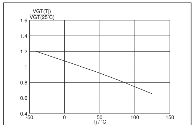
Fig.6. Normalised gate trigger voltage V_{GT}(T_j) / V_{GT}(25\text{ °C}) , versus junction temperature T_j .
