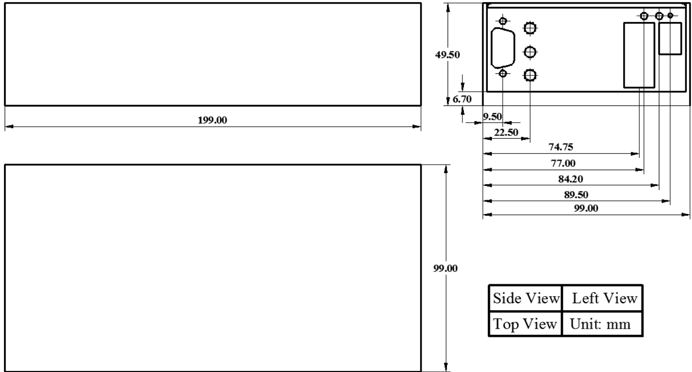
Figure 29. Mechanical Dimensions
