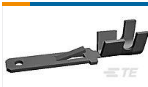
TE Part #42460-2 FF 250 TAB 18-14AWG TPBR
