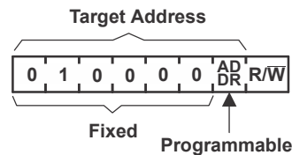
Figure 8-6. TCA6416A Address
