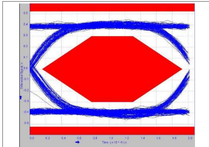
Figure 11. 480-Mbps USB 2.0 Eye Pattern With No Device
