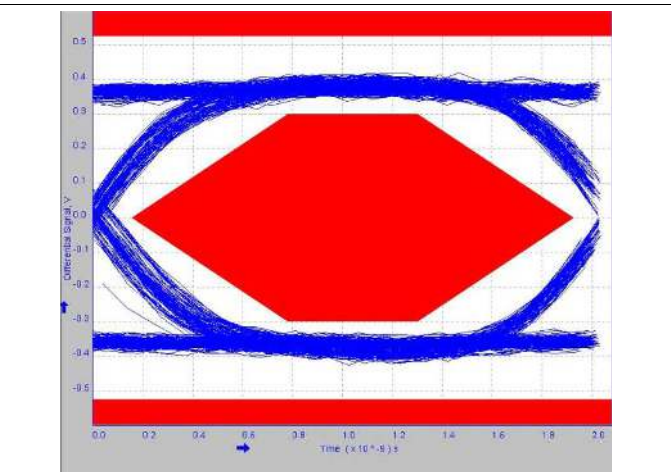
Figure 12. 480-Mbps USB 2.0 Eye Pattern for USB Switch
