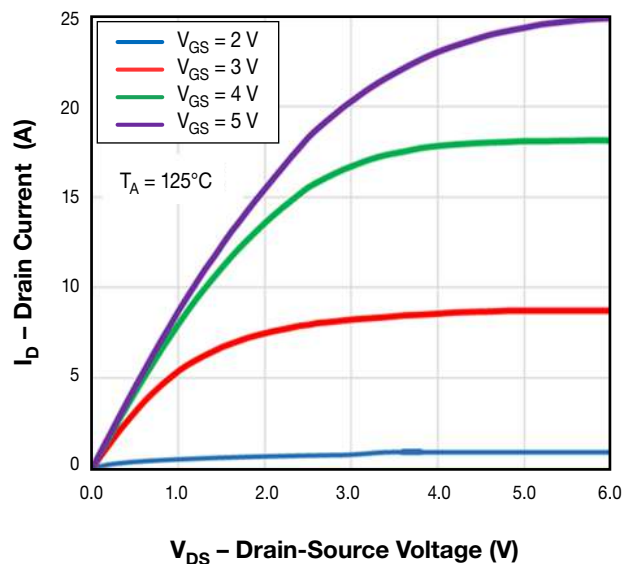
Figure 5. Typical Output Characteristics
