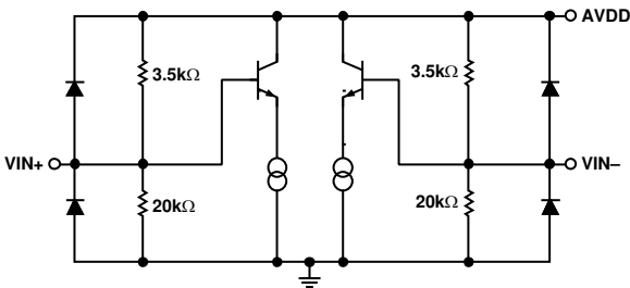
Figure 5. Analog Inputs
