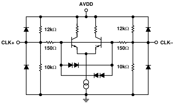
Figure 4. Clock Inputs
