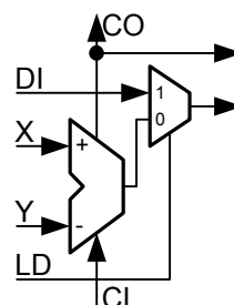
Figure 71. Preloadable Subtractor.
