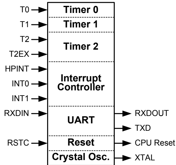
Figure 65. Embedded Accelerated 8051 microcontroller sideband signals.
