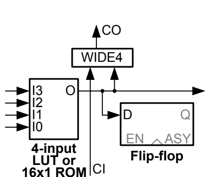
Figure 66. Four-input logic function.
