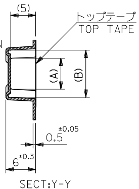
SECT: Y-Y
