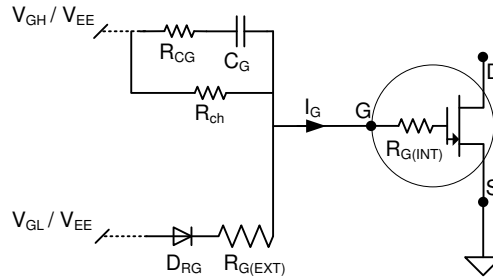
Figure 23: Primary gate drive circuit passive components with series gate resistor Schottky rectifier.
