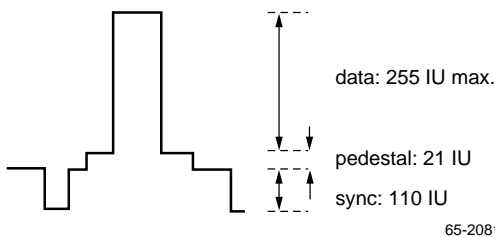
Figure 2. GBR/Y DAC Output Levels in Current Units
