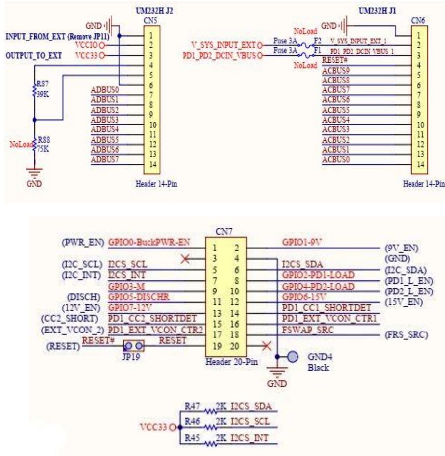
Figure 10 - Interfaces and Connectors
