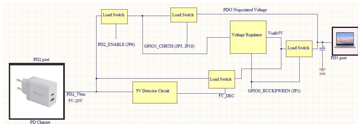
Figure 11 - Pass-through Block Diagram
