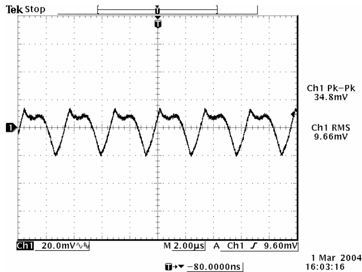
Ripple and noise at full load, 3.3 V input, 2.5 V output
