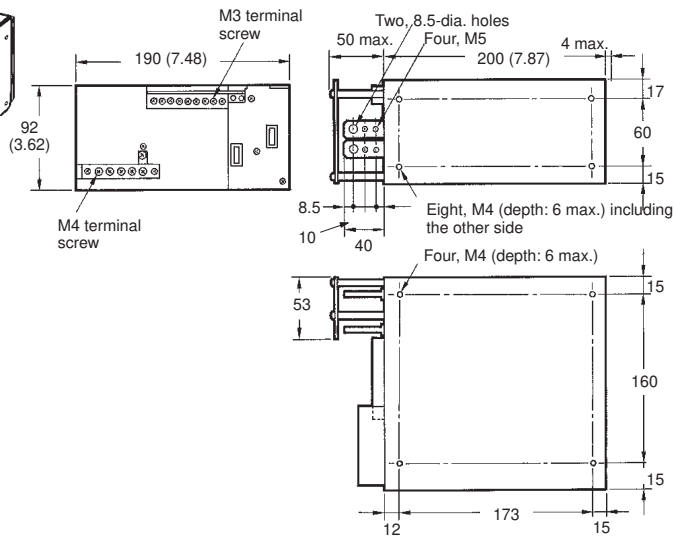
Mounting Holes Side View
