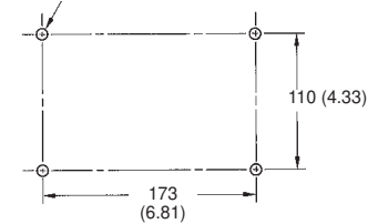
Mounting Holes
