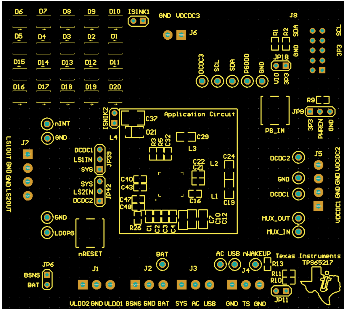
Figure 5. Layout - Silkscreen
