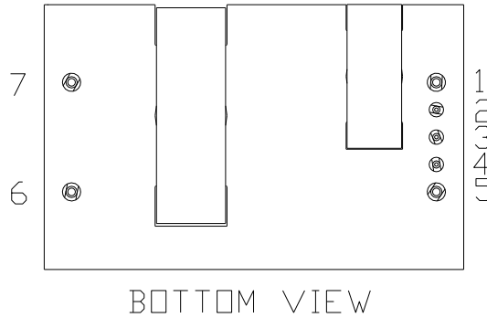
Figure 53. 0RQB-50Y05L/0 Pins
