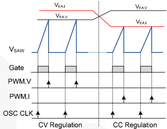
Figure 25. PWM Operation for CC and CV
