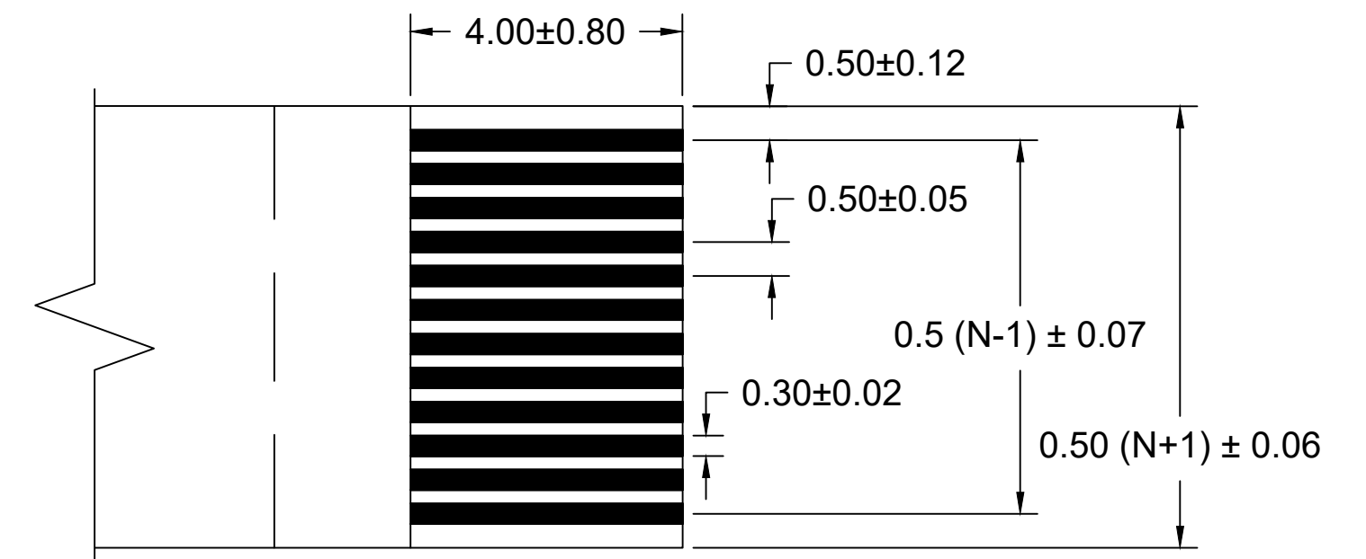
END TAIL DETAIL SCALE 10:1
