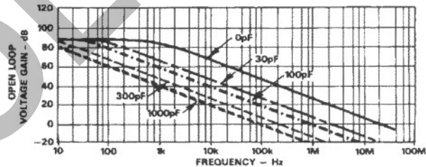
Figure 7. Open Loop Frequency Response for Various C c 's
