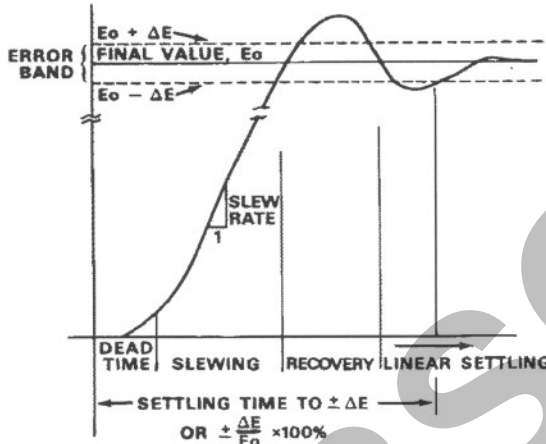
Figure 1. Settling Time
