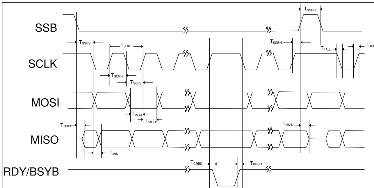
Figure 12-2 SPI Timing
