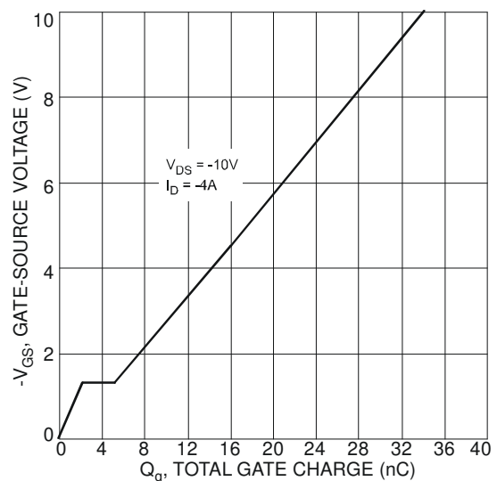
Fig. 12 Gate-Charge Characteristics
