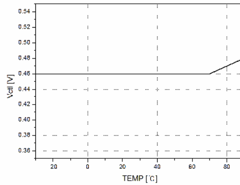
Figure 12. CT Low Voltage vs. Temperature
