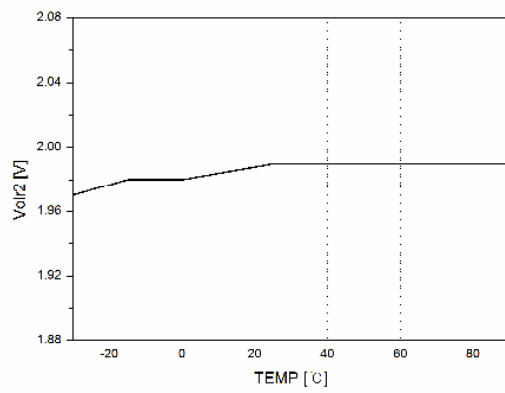
Figure 30. Open Lamp Regulation Voltage 2 vs. Temperature
