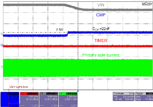
Figure 61. CMP-High Protection Disabled by a Pull-Down Resistor
