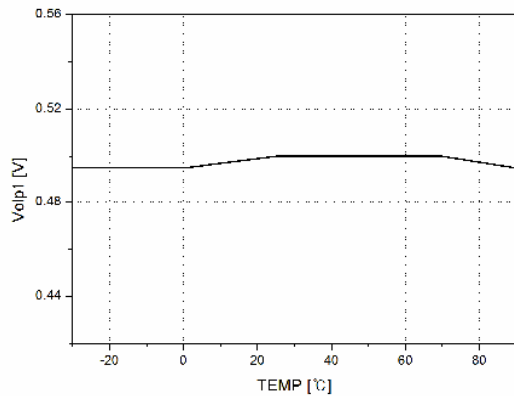
Figure 25. Open-Lamp Protection Voltage 1 vs. Temperature
