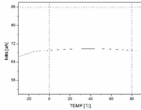
Figure 24. OLR Error Amplifier Sink Current vs. Temperature
