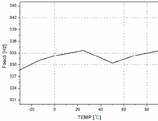
Figure 13. Burst Dimming Frequency vs. Temperature
