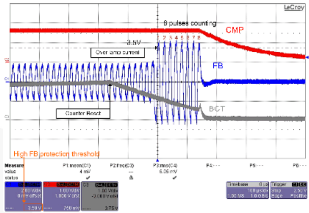
Figure 62. FB-High Protection
