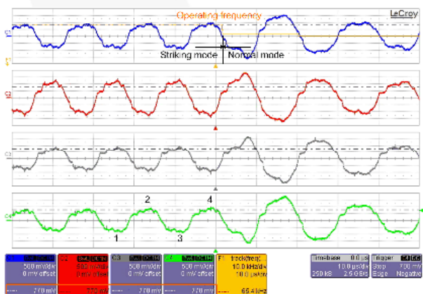
Figure 53. Mode Change from Striking to Normal
