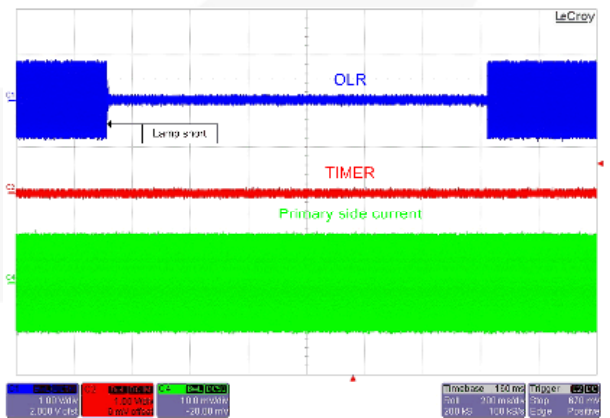
Figure 59. Short-Lamp Protection Disable in DCR Mode
