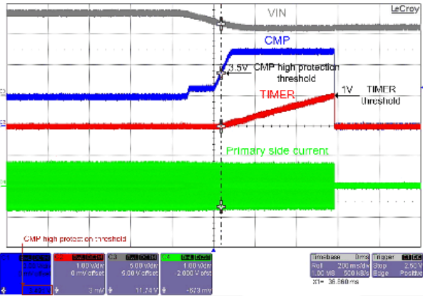
Figure 60. CMP-High Protection
