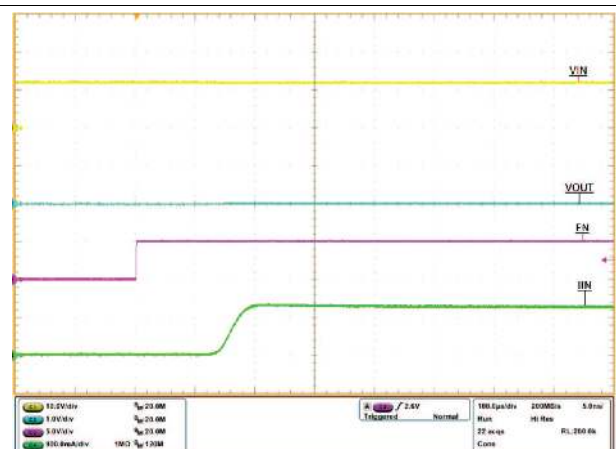
V_{IN} = 12\text{ V} , C_{OUT} = 1\ \mu\text{F} , R_{ILM} = 487\ \Omega
