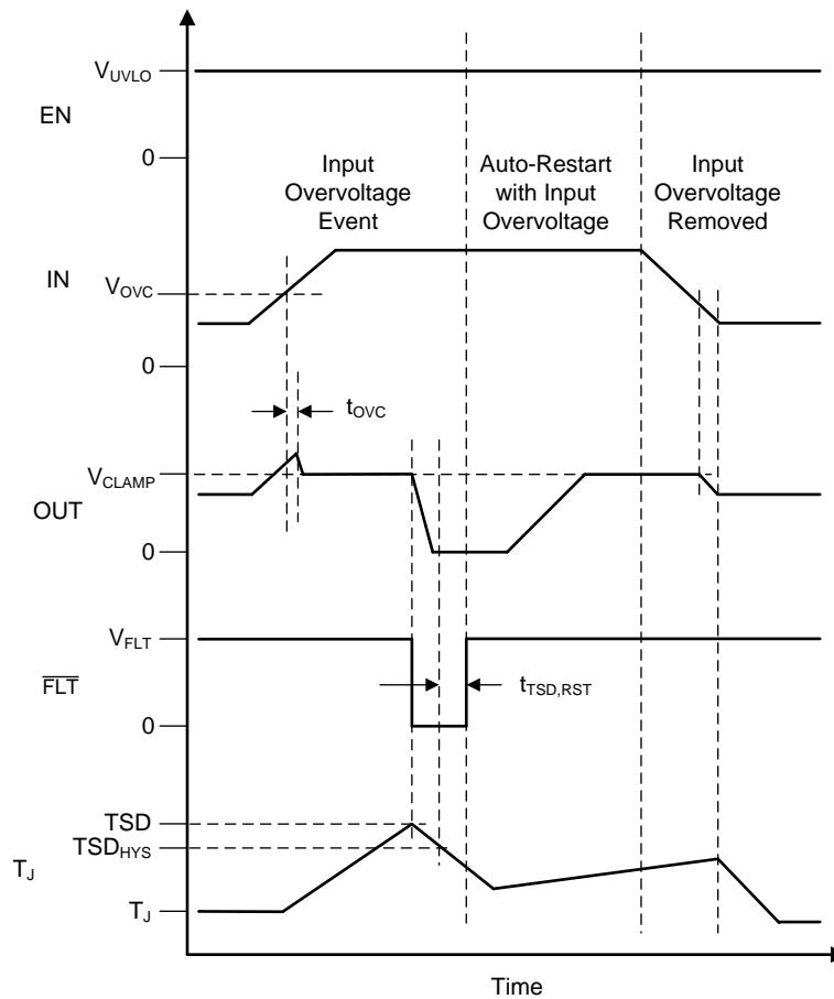
Figure 49. TPS2595xx Overvoltage Clamp Response (Auto-Retry)
