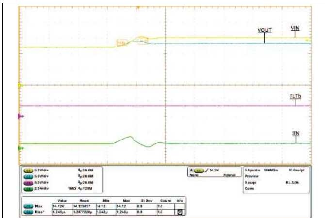
V IN Stepped from 12 V to 15 V, C OUT = 1 μF, R ILM = 487 Ω, FLT b = 3.3 V through 10 kΩ, R OUT = 20 Ω
