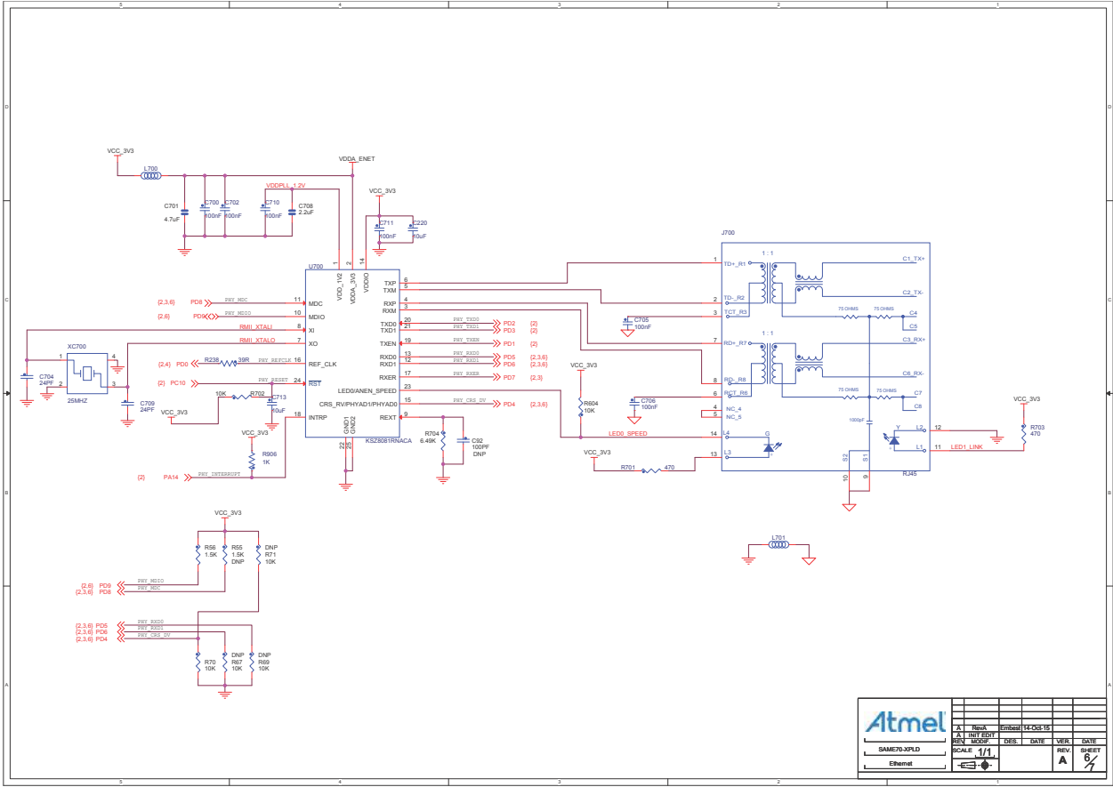
Figure 5-6 Ethernet 10/100
