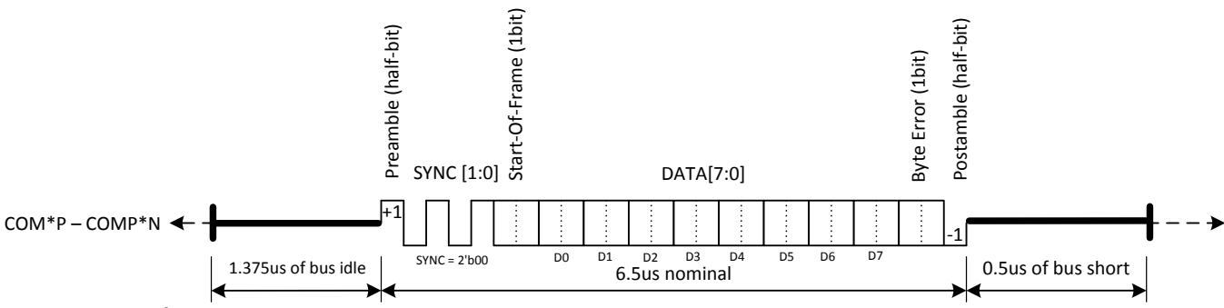
Figure 28. Daisy Chain Protocol Structure
