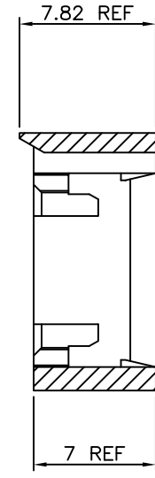
SECTION B-B
