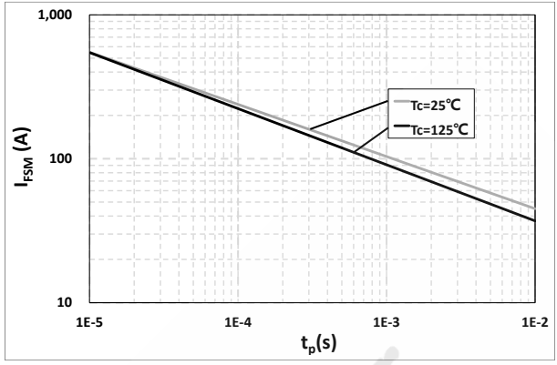
Figure 8. Non-repetitive peak forward surge current versus pulse duration (sinusoidal waveform)
