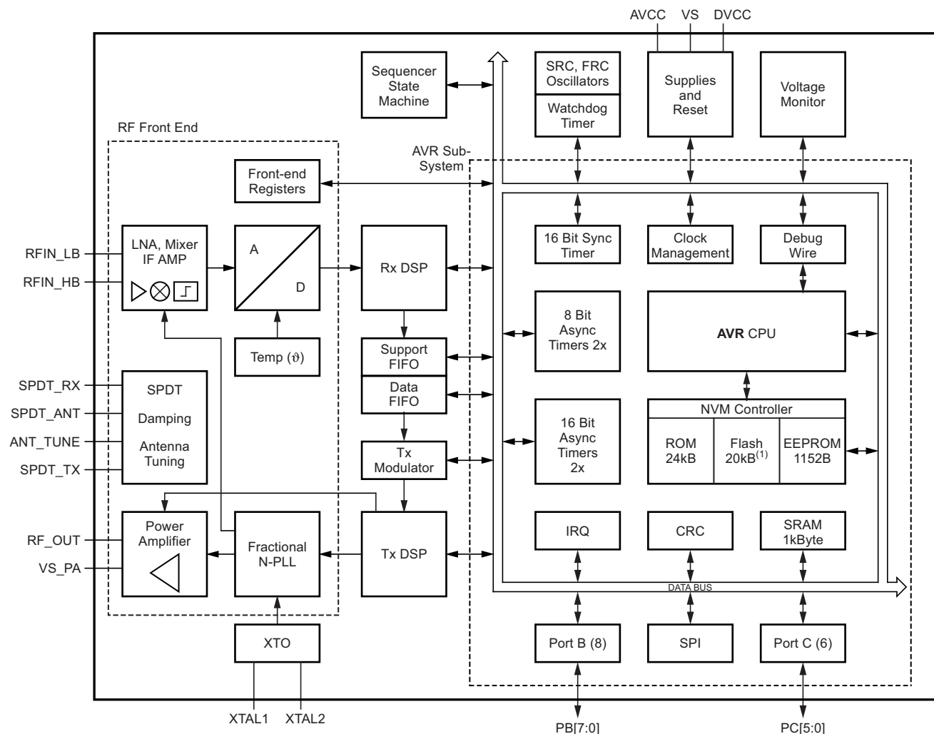
Figure 3-1. Block Diagram
