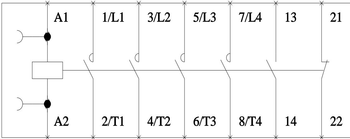
LENO0C004 Wiring Diagram
