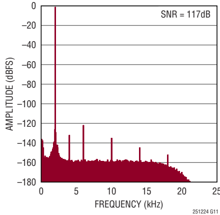
128k Point FFT f_{SAMPL} = 1.6\text{Mps} , f_{IN} = 2\text{kHz} , DF = 32
