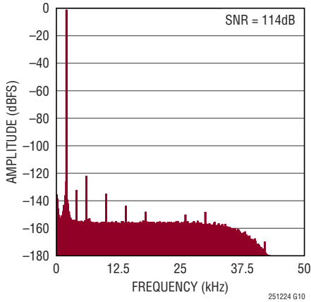
128k Point FFT f_{SAMPL} = 1.6\text{Mps} , f_{IN} = 2\text{kHz} , DF = 16
