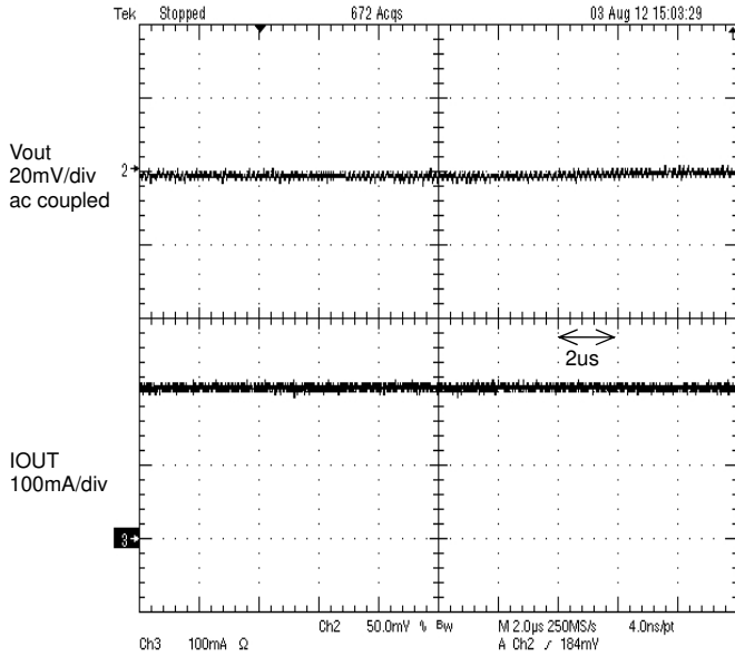
Figure 45 PWM/PFM Auto mode Operation Iout=200mA
