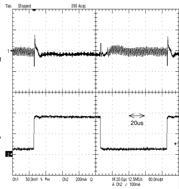
Figure 8. Load transient response 50mA to 350mA tr=100ns , MODE : Low
