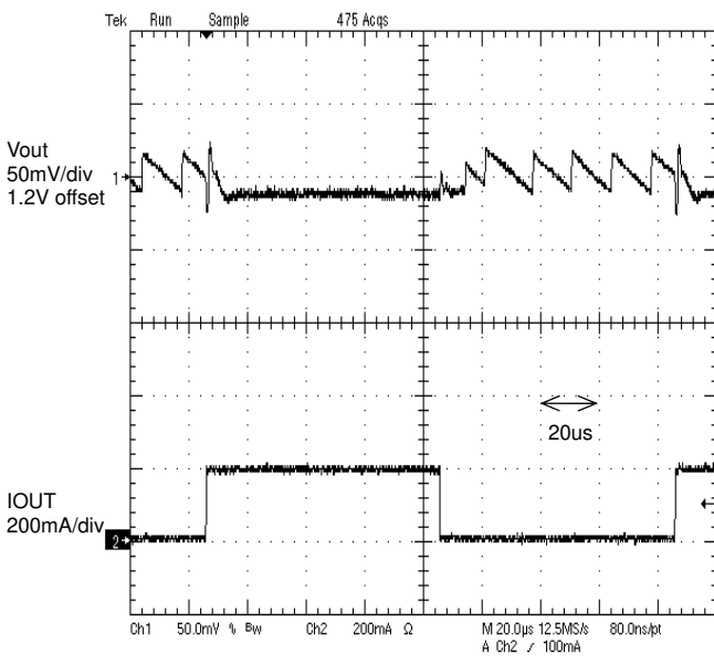
Figure 7. Load transient response 5mA to 200mA tr=100ns , MODE : Low
