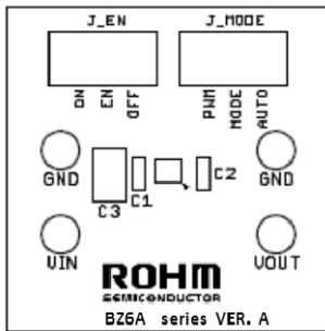
Figure 54. PCB layout (Mount side)
