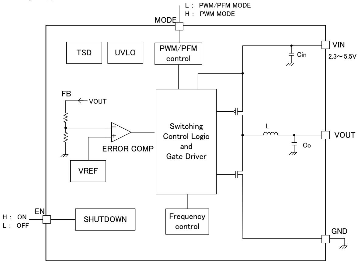
Figure 3. Block Diagram(s)
