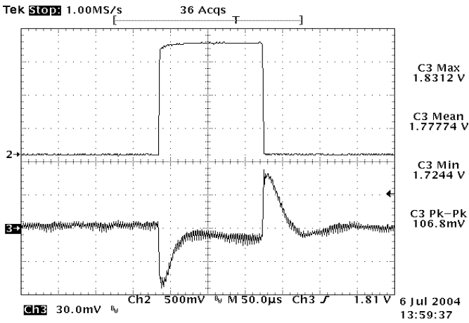
Figure 21: Typical transient response to step load change at 10A/μs from 50% to 75% and 75% to 50% of I o , max at 12V in , 1.8V out
