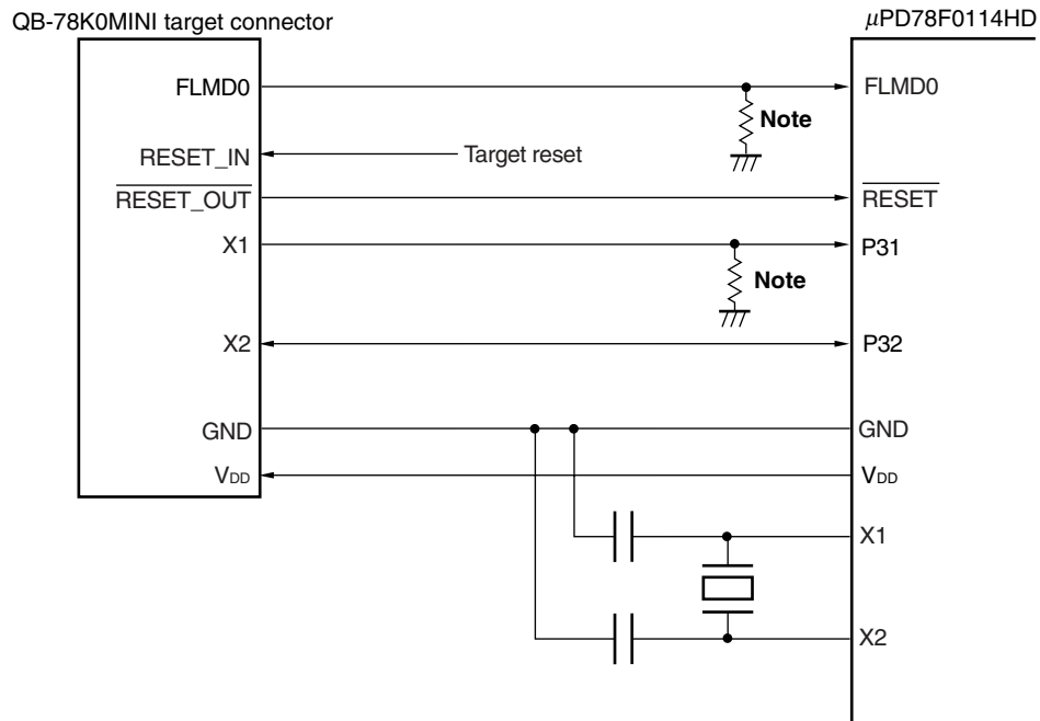
Figure 24-2. Connection Example of QB-78K0MINI and \mu PD78F0114HD (When P31 and P32 Are Used)
