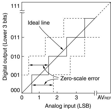
Figure 11-15. Zero-Scale Error
