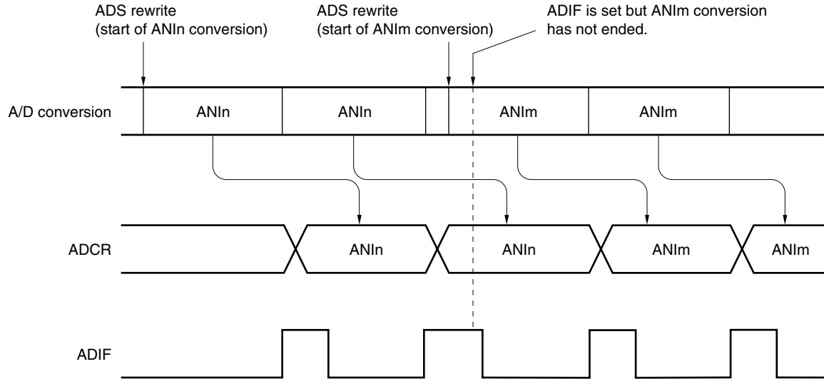
Figure 11-20. Timing of A/D Conversion End Interrupt Request Generation
