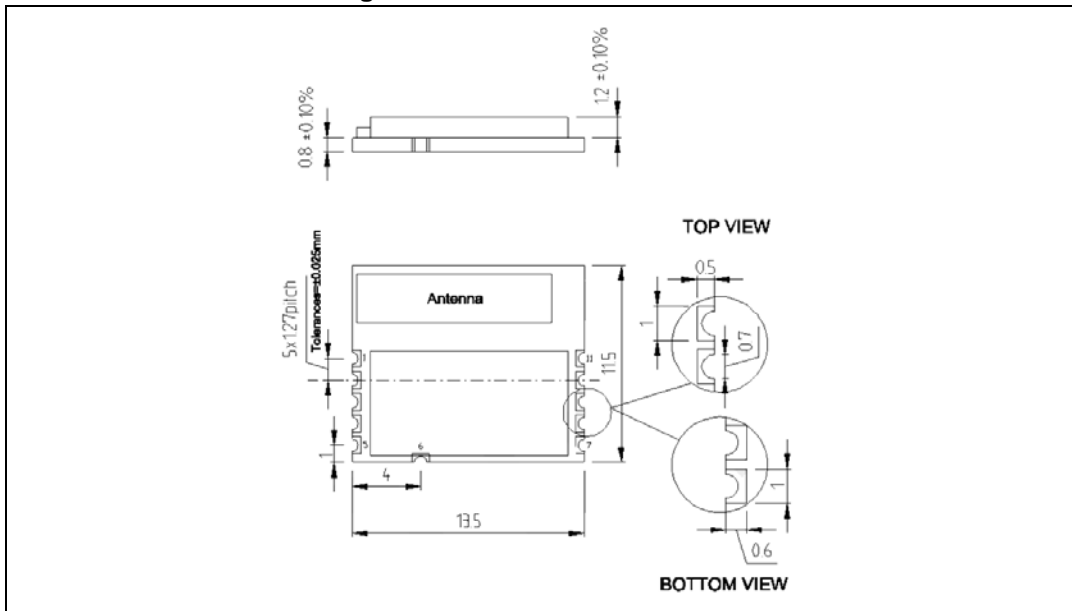
Figure 4. Mechanical dimensions
