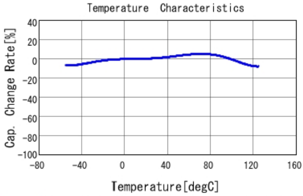
GRT188R70J225KE13 C-Temp. capchange, DC0.0V, AC0.5
