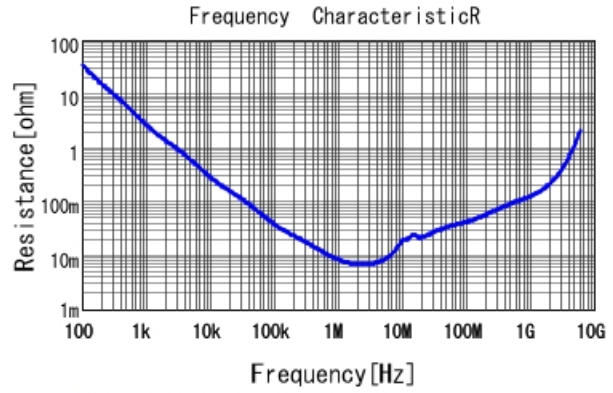
GRT188R70J225KE13 R DCOV, 25degC
