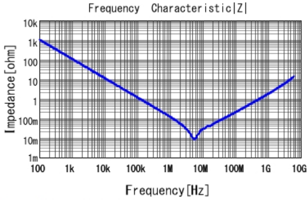
GRT188R70J225KE13 |Z| DCOV, 25degC
