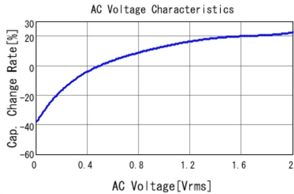
GRT188R70J225KE13 C-AC Voltage capchange, DCOV, 25
