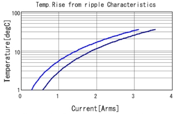
GRT188R70J225KE13 Temp. rise — 500kHz — 1MHz
