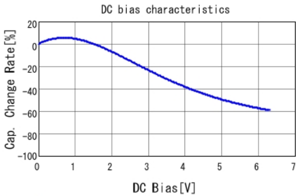
GRT188R70J225KE13 C-DC bias capchange, 25.0degC, A
