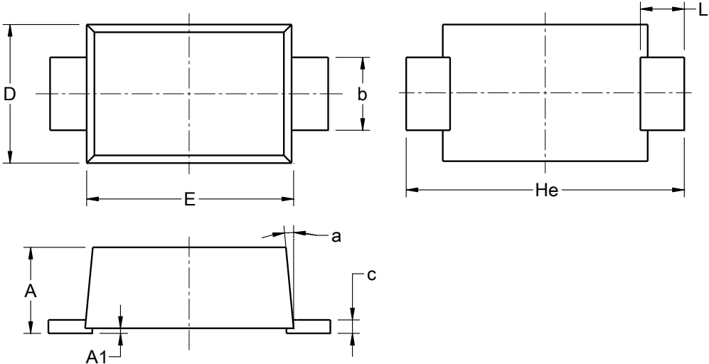
DO-219AA
