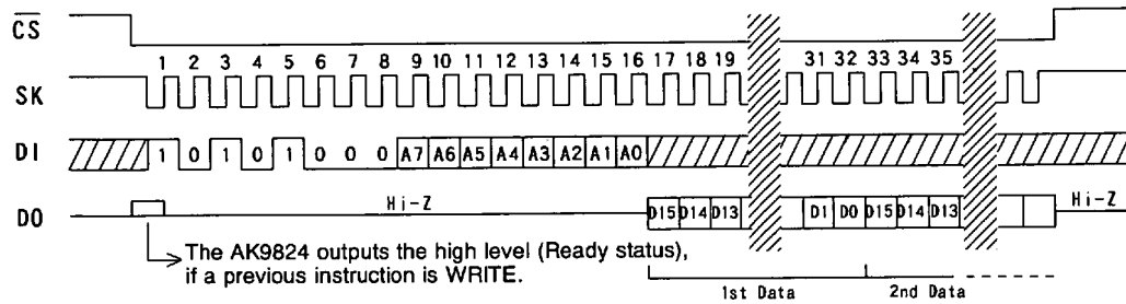
READ (AK9824)
