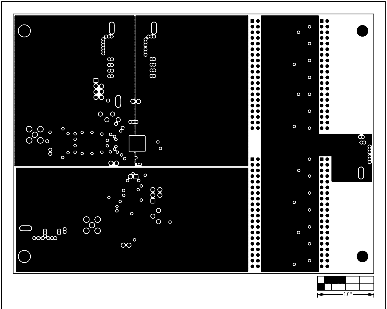
Figure 5. MAX1213N/MAX1214N EV Kit PC Board Layout—Power Plane (Layer 3)
