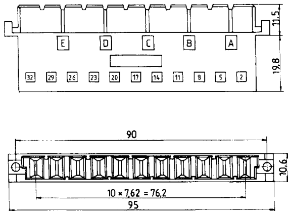
Drawing
