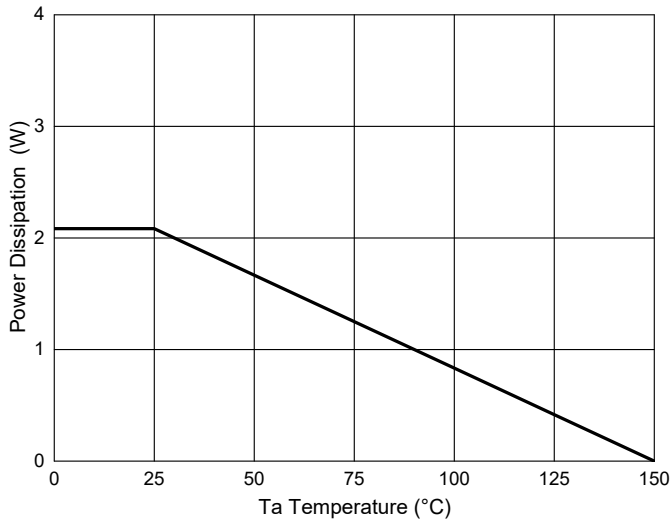
Fig.11-PD Dissipation
