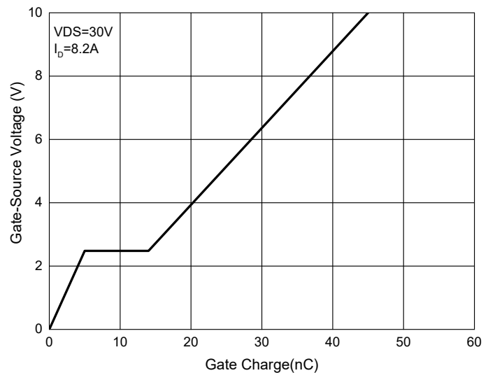
Fig. 6 - Gate Charge
