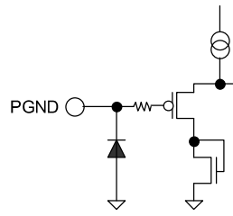
Figure 39. PGND
