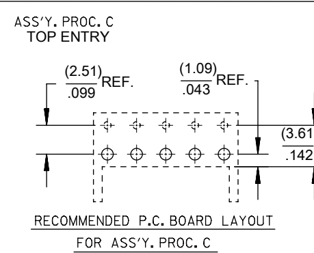
RECOMMENDED P.C. BOARD LAYOUT FOR ASS'Y. PROC. C
