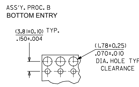
RECOMMENDED P.C. BOARD LAYOUT FOR ASS'Y. PROC. B
