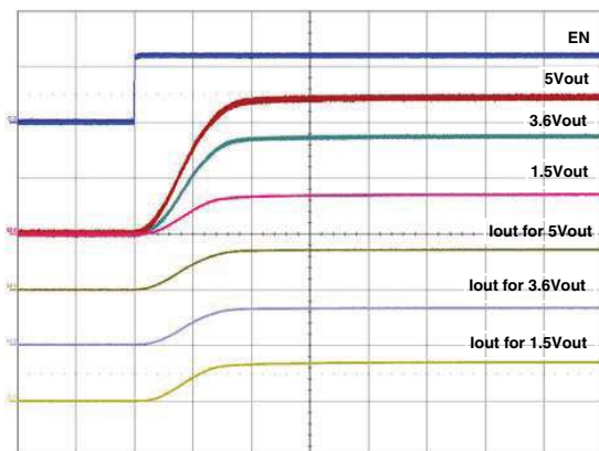
Fig. 22 - Typical Turn-On Delay, Rise Time C OUT = 200 μF, C IN = 4.7 μF, I OUT = 1.5 A
