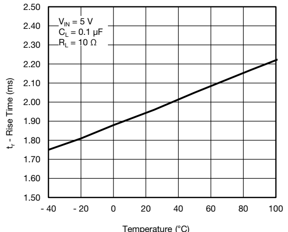
Fig. 16 - Rise Time vs. Temperature
