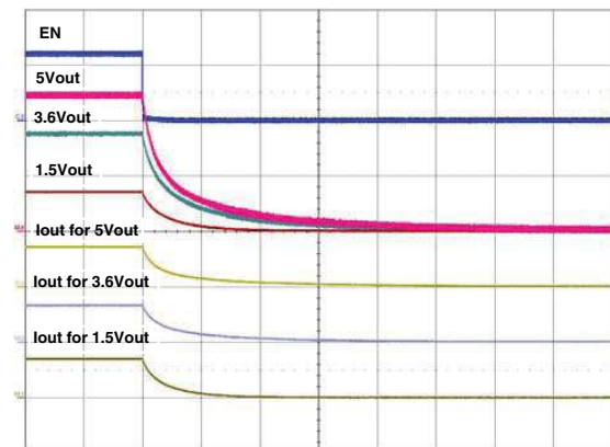
Fig. 25 - Typical Fall Time C OUT = 200 μF, C IN = 4.7 μF, I OUT = 1.5 A
