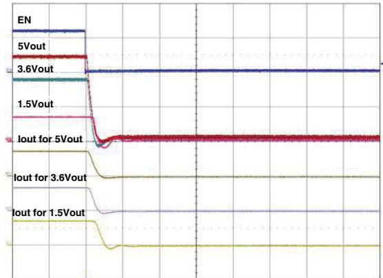
Fig. 23 - Typical Fall Time C OUT = 0.1 μF, C IN = 4.7 μF, I OUT = 1.5 A
