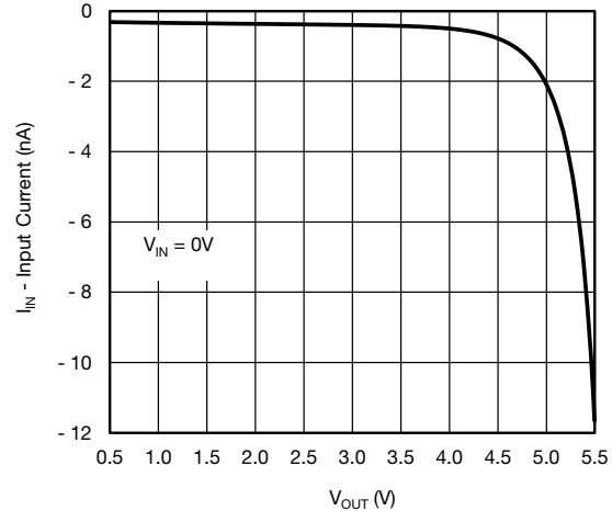
Fig. 15 - Reverse Blocking Current vs. Output Voltage
