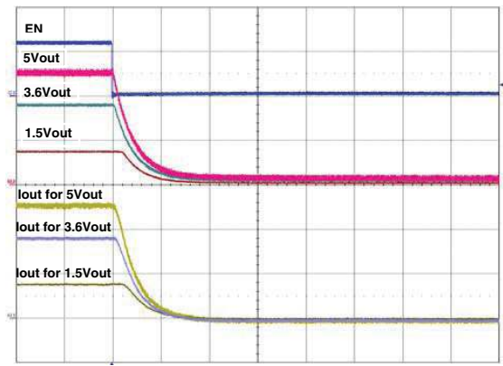
Fig. 24 - Typical Fall Time C OUT = 0.1 μF, C IN = 4.7 μF, R OUT = 10 Ω
