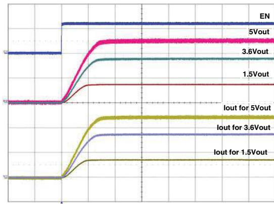
Fig. 21 - Typical Turn-On Delay, Rise Time C OUT = 0.1 μF, C IN = 4.7 μF, R OUT = 10 Ω
