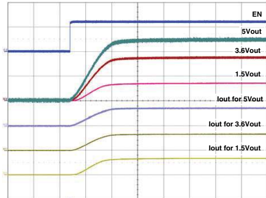
Fig. 20 - Typical Turn-On Delay, Rise Time C OUT = 0.1 μF, C IN = 4.7 μF, I OUT = 1.5 A
