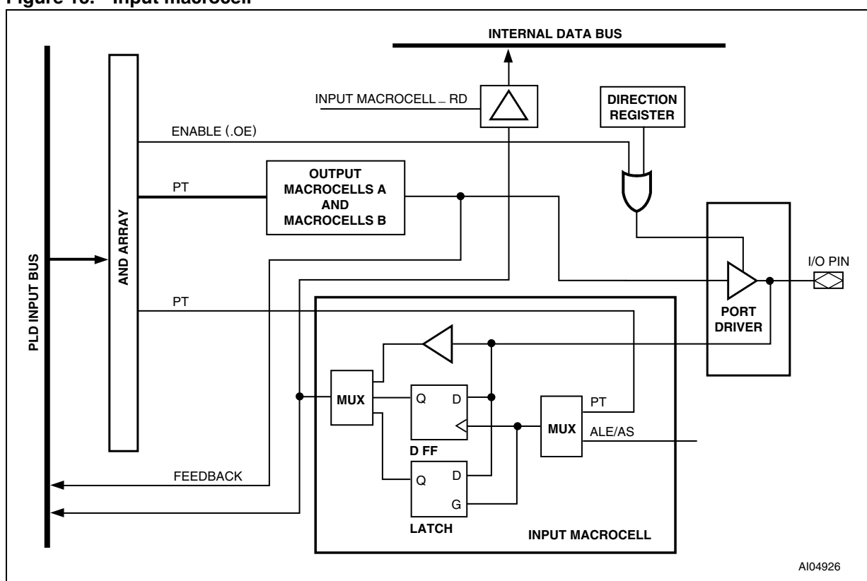
Figure 15. Input macrocell
