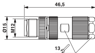
Dimens. drawing: M12 connectors
