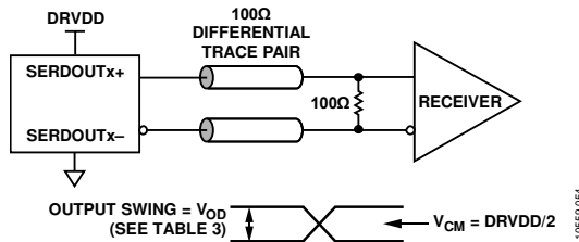
Figure 58. DC-Coupled Digital Output Termination Example
