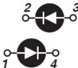
Figure 2 • Anti-parallel MSC2X50SDA120J
