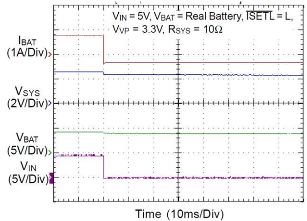
V_{IN} Removal
