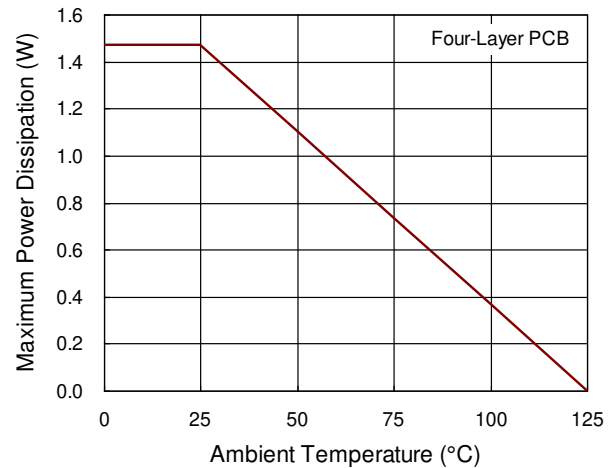
Figure 2. Derating Curves for RT9519A Package
