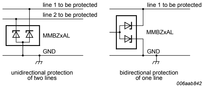
Fig. 15. Application diagram
